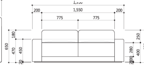
2인소파 FRONT VIEW
